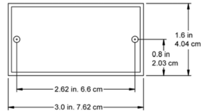
Mounting Dimensions
